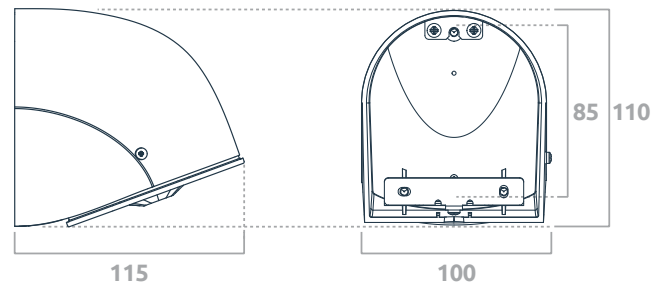
6 Surface mount
