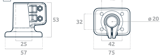
7 Rod mount
